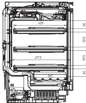
KWTUS7054F, interior dimensions (installation drawings)
