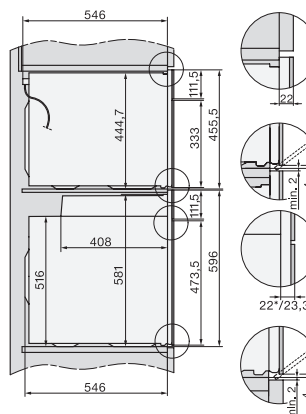
H2xxx-1 B/BP/E/EP, H7xxx B/BP/BM/BMX, installation drawings
