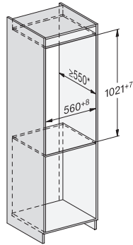
K7216E, built-in (*footnote) (installation drawings)
